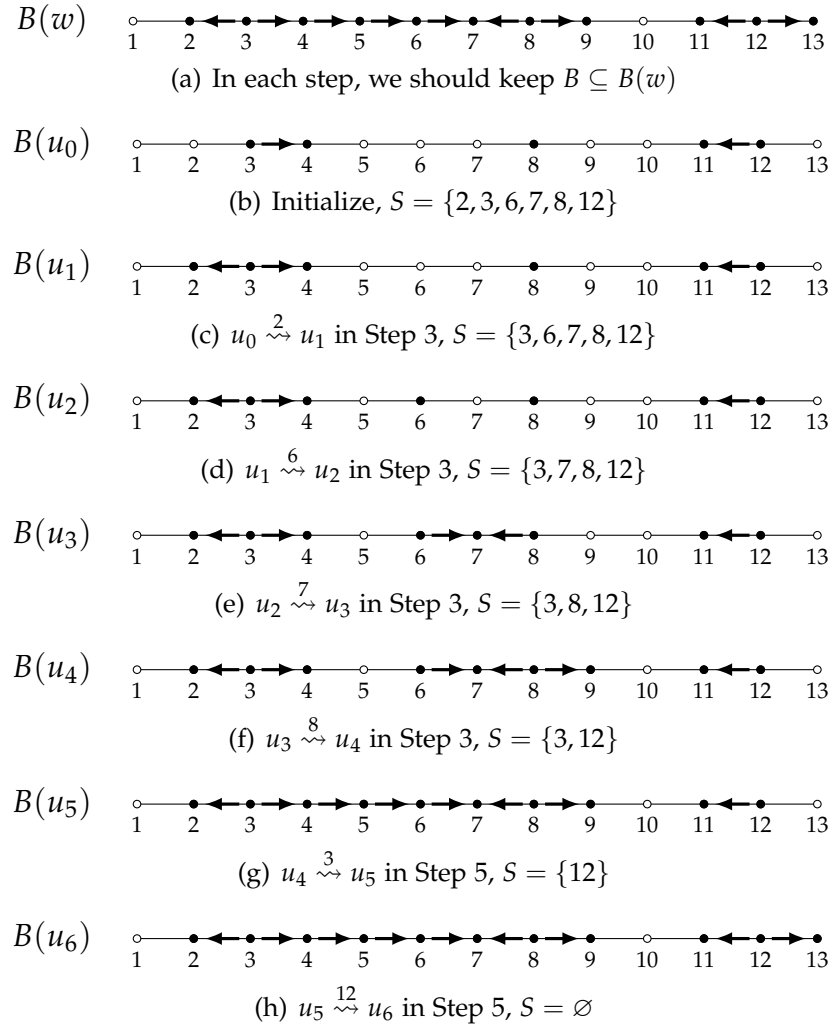
Figure 7: An example for Algorithm 1, that results in a boolean insertion path u = u_0 \xrightarrow{2} u_1 \xrightarrow{6} u_2 \xrightarrow{7} u_3 \xrightarrow{8} u_4 \xrightarrow{3} u_5 \xrightarrow{12} u_6 = w .
