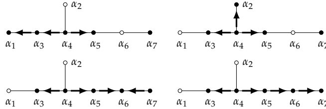
Figure 3: The boolean diagrams B(v) for all the boolean elements v satisfying s_3 s_5 s_4 s_7 = u \xrightarrow{\alpha_4} v with a non-equivariant insertion step.
