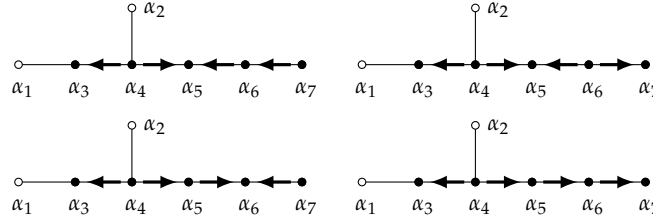
Figure 4: The boolean diagrams B(v) for s_3s_5s_4s_7 = u \xrightarrow{\alpha_6} v .
